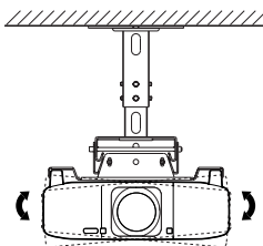
Horizontal roll adjustment
