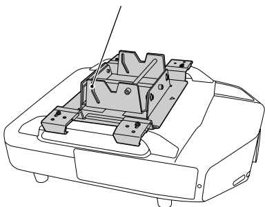
Align the screw holes on the handles and on the hooks.
