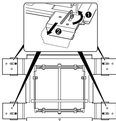
Vertical tilt adjustment hole
